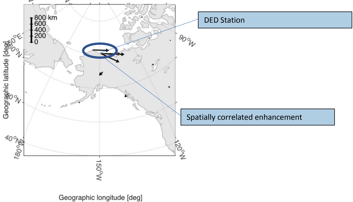
Goelectric field distribution 2015-03-17T13:33:00 UT. Max. IEI: 3.46 V/km.
